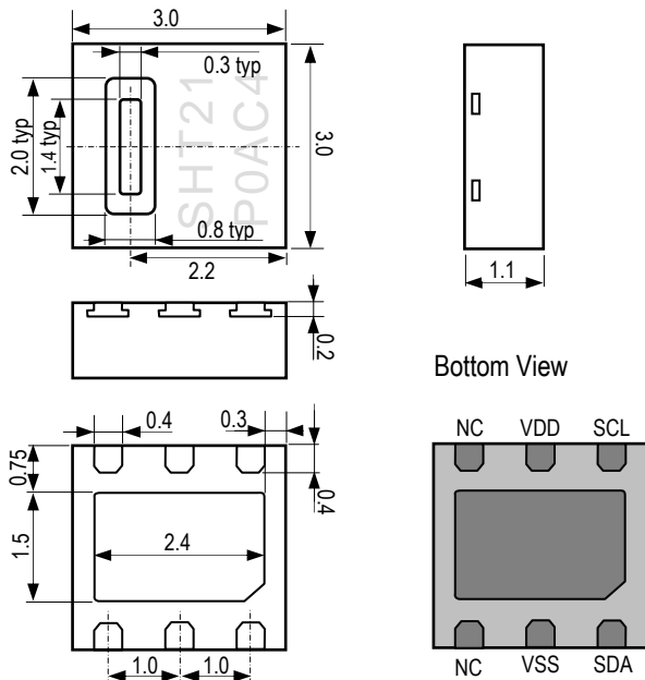
Figure 1: Drawing of SHT21P sensor package, dimensions are given in mm (1mm = 0.039inch), tolerances are \pm 0.1 mm. The die pad (center pad) is internally connected to VSS. The NC (center pad) is internally connected to VSS. The NC pads must be left floating. Numbering of E/O pads starts at lower right corner (indicated by notch in die pad) and goes clockwise (compare Table 2).
