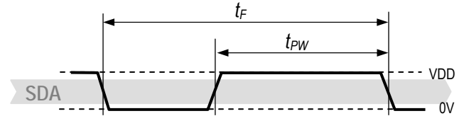
Figure 10 PWM signal. Base frequency runs constantly at approximately 120 Hz, hence t_F is about 8.3ms. The signal is provided on t_{PW} as a ratio of t_F .
